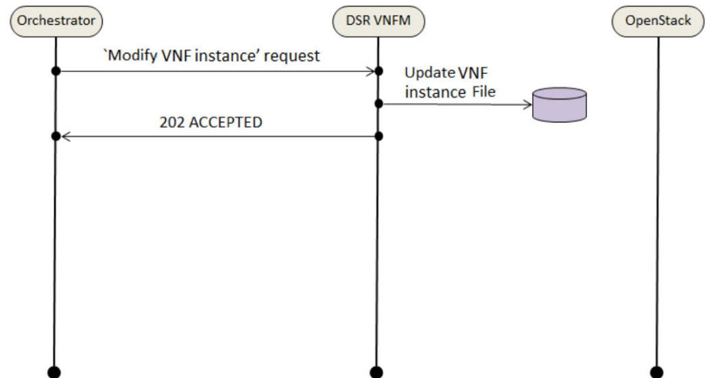
Figure 9-3 Modify VNF Instance Request
